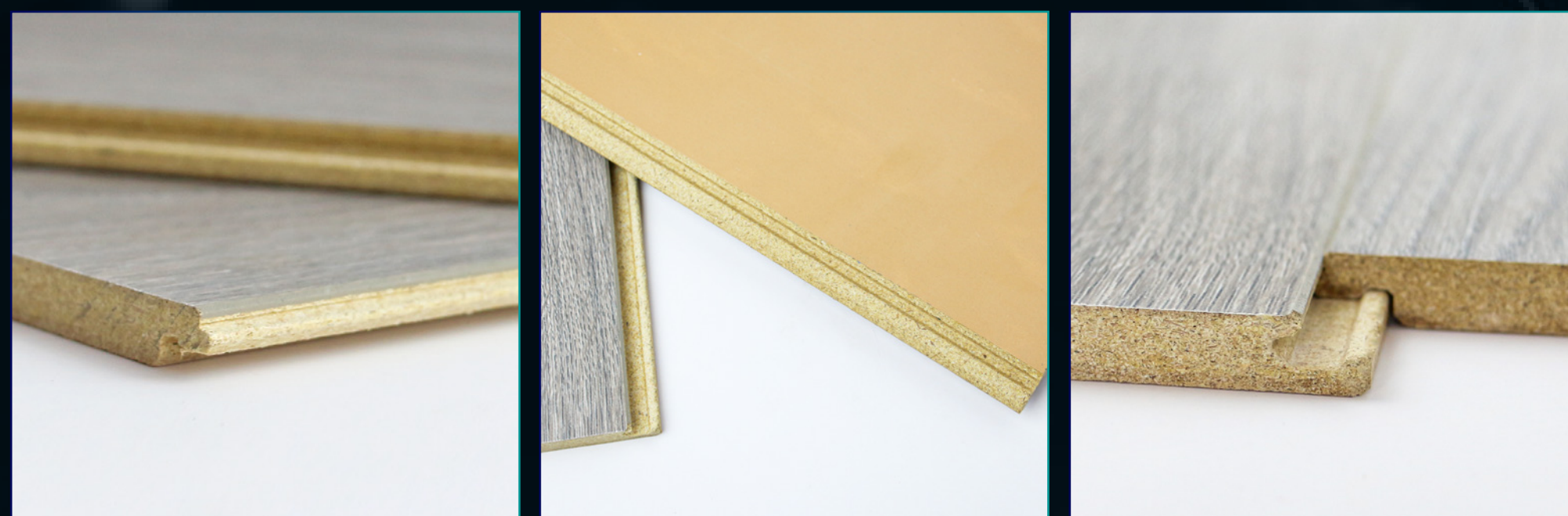
Valinge 2G-FD click system
